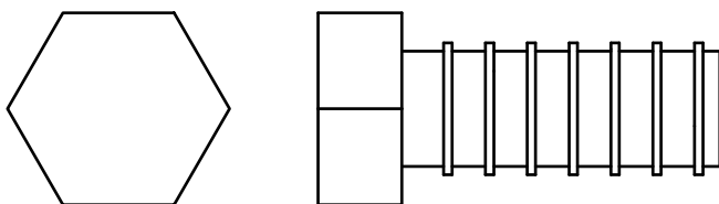
(A6)HIGH STRAIN HEX BOLT 5/8"X1-1/2"L PARTIAL QTY.2
